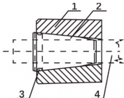
1.Anchor ring 2.Anchor clamp 3.Steel wire loop 4.Anchor cable(steel strand)
