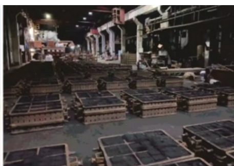
Mechanical pouring production line
