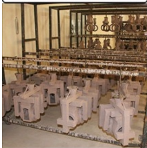
Shell Drying
