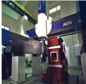
Tri-coordinate test
