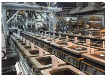
AUTOMATIC CASTING
