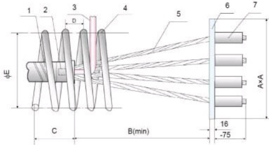
1.Duct 2. Restraining ring 3. Vent 4. Spiral reinforcement 5. Strand 6. Dead-end bearing plate 7. Swaged end
