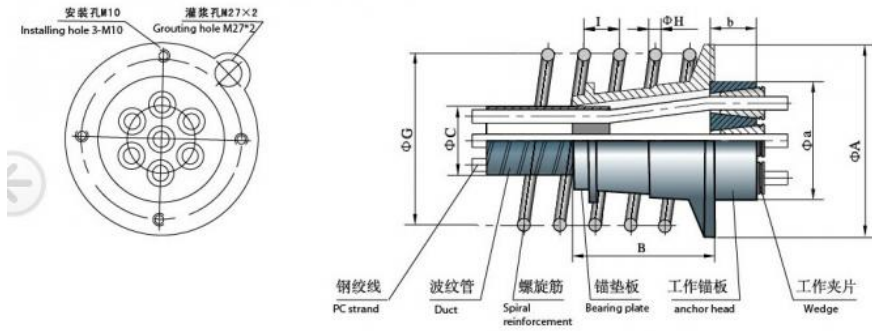
LQM15、LQM13型张拉端总成构造图 Structural chart of LQM15 and LQM13 tensioning end assembly
